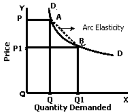
Fig. 8: Arc Elasticity
